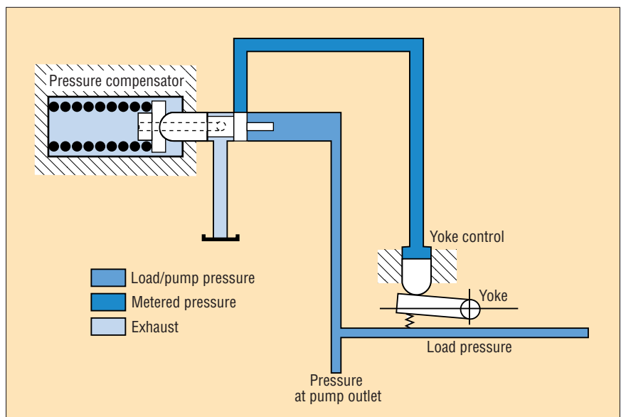
Fig. 12. Schematic of typical proportional pump pressure compensator control.
