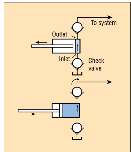
Fig. 1. Reciprocating pump.
