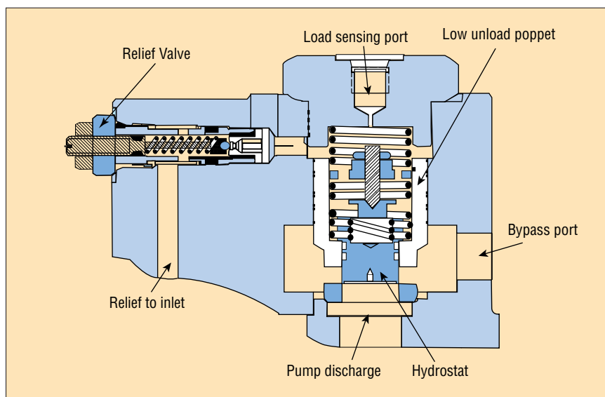
Fig. 22. This cutaway shows combined control, which has an adjustable hydrostat contained within the unloader control. Locating the hydrostat within the low-unload control allows all piston areas to operate from a single load-response signal. It is intended for applications using large pumps where secondary flow bypasses to tank.
