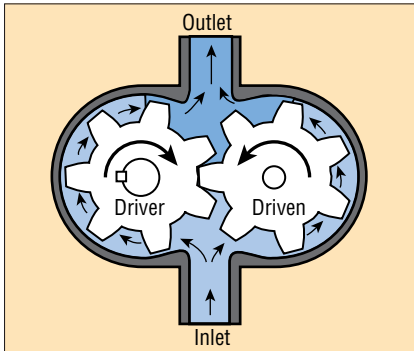
Fig. 2. Spur gear pump.
