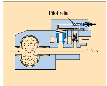
Fig. 21. Combined control is achieved by incorporating a pilot relief, which causes the hydrostat to act as the main stage of a pilot-operated relief valve.
