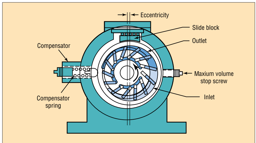
Fig. 7. Variable displacement, pressure compensated vane pump.
