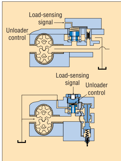
Fig. 20. Unloader control has been added to the load-sensing gear pump. The control uses a poppet or a plunger to allow maximum flow at the minimum pressure drop across the unloader with minimal control movement.
