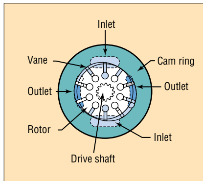
Fig. 6. Balanced vane pump.
