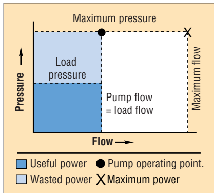
Fig. 13. Pressure-flow curve of variable-displacement hydraulic pump equipped with pressure compensation.
