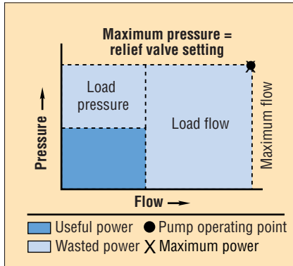
Fig. 10. Pressure-flow curve of hydraulic system with fixed-displacement pump.
