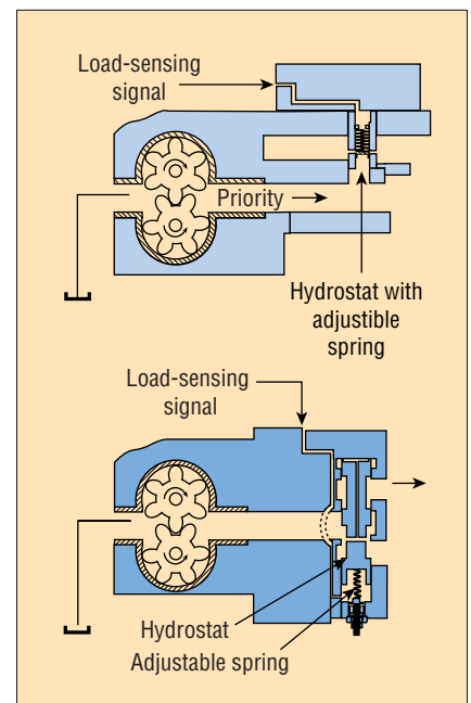
Fig. 19. Load sensing gear pumps with two different types of hydrostats installed. The spring adjustment allows tuning pressure drop for different manufacturers' valves or line lengths.
