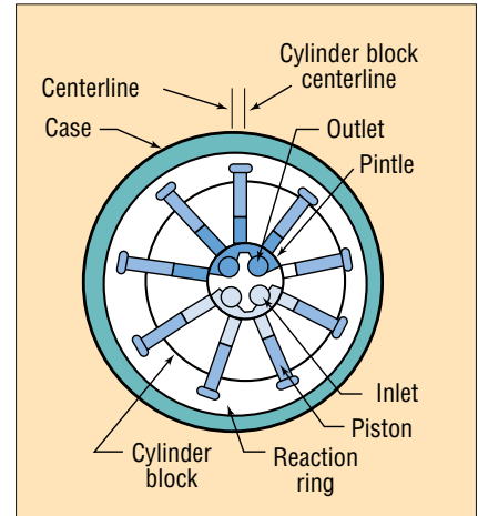
Fig. 9. Radial-piston pump.
