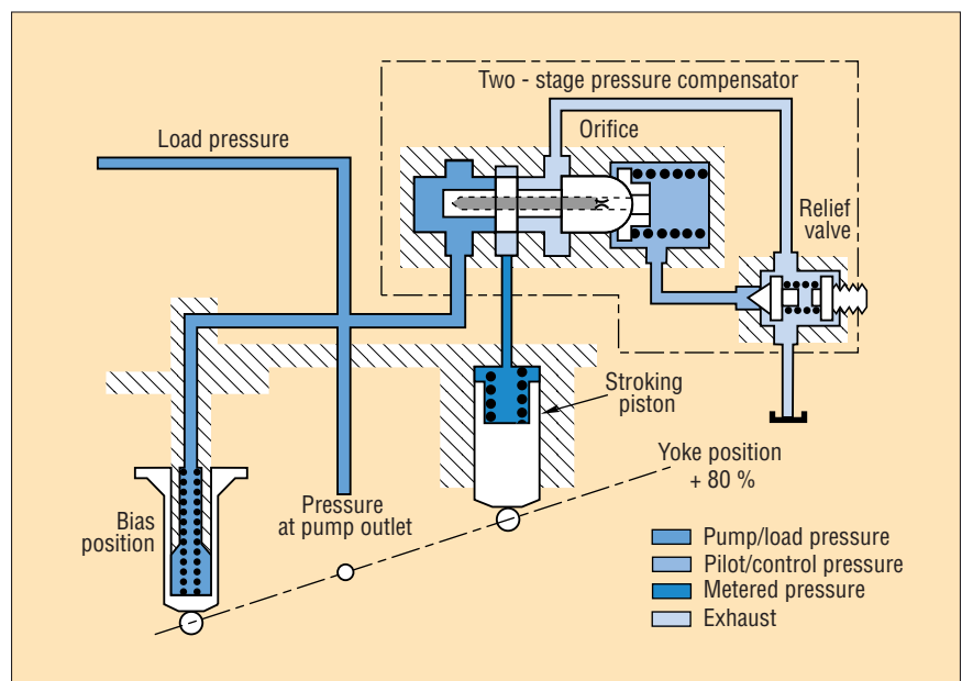
Fig. 14. Schematic of pump two-stage compensator control.
