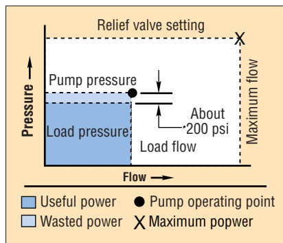
Fig. 17. Pressure-flow curve of pump with load-sensing control.
