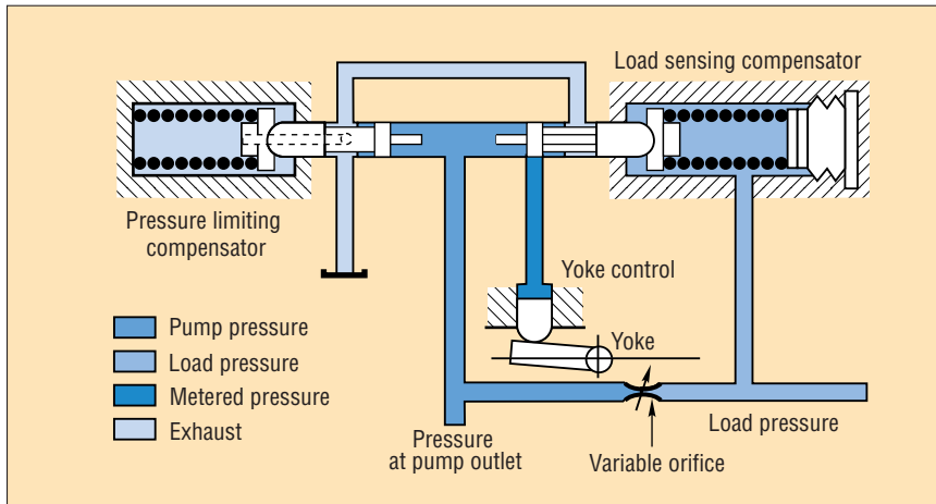
Fig. 18. Schematic of pump control that provides load sensing and pressure limiting.
