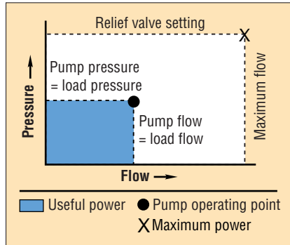
Fig. 11. Pressure flow curve of variable-displacement hydraulic pump with ideal flow and pressure compensation.
