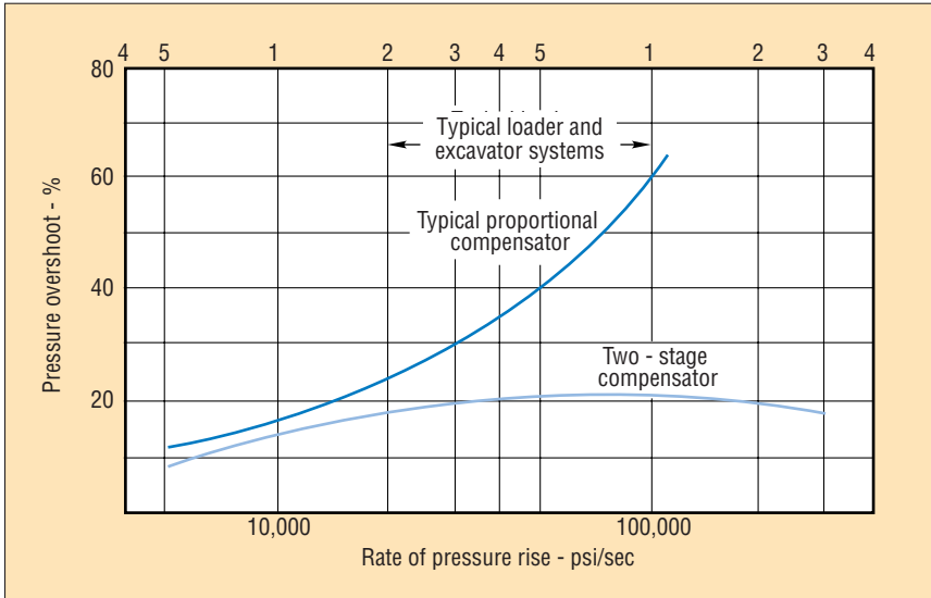
Fig. 15. Typical performance of a single- and two-stage pressure compensation.
