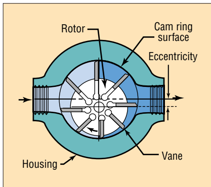
Fig. 5. Basic (unbalanced) vane pump.
