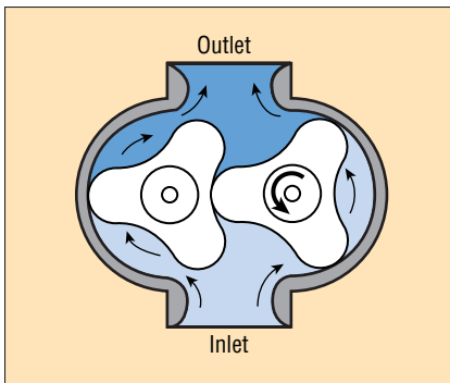
Fig. 3. Lobe pump.
