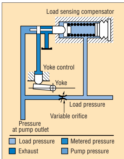
Fig. 16. Schematic of proportional pump compensator that provides load-sensing capability.
